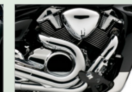
1783cm 3 liquid-cooled 4-stroke DOHC V-twin engine
